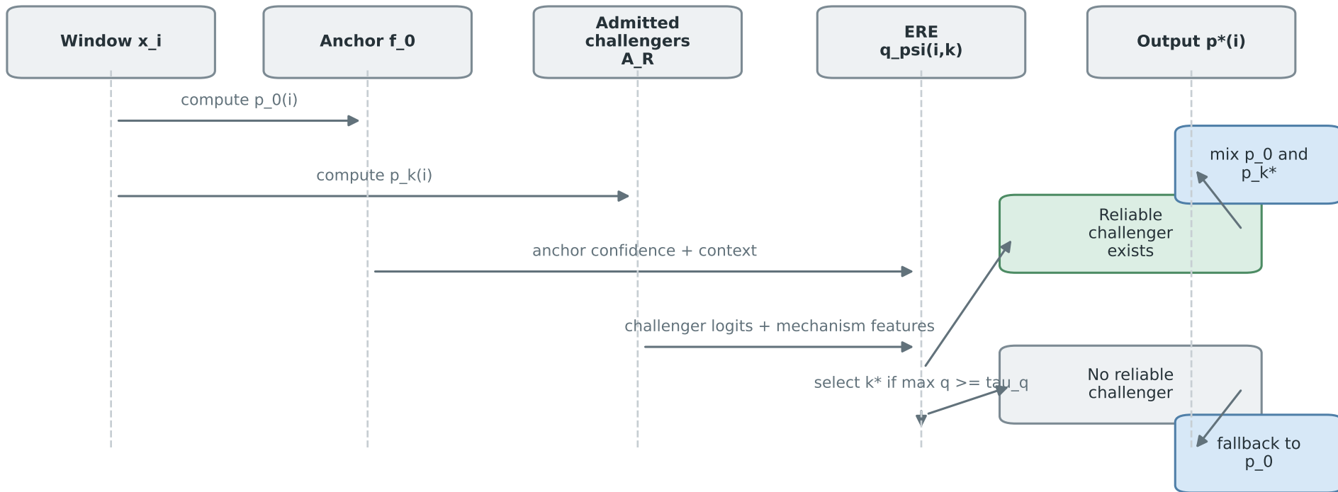
Figure 3. Anchor-Challenger Deployment Rule
