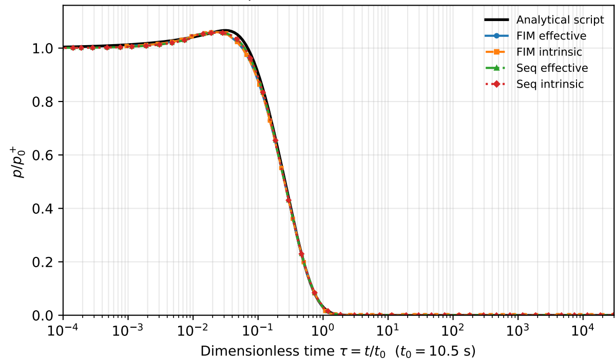
Fracture pressure at center/no-flow axis
