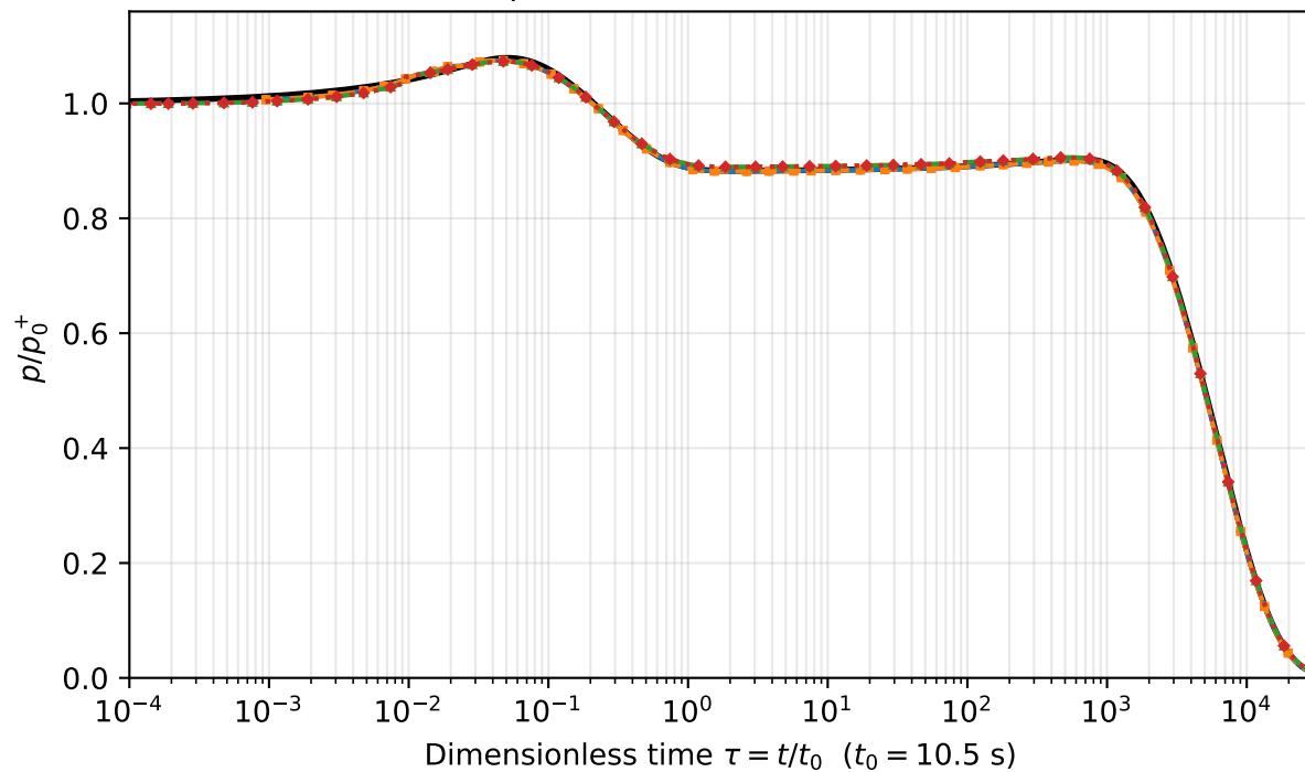
Matrix pressure at center/no-flow axis
