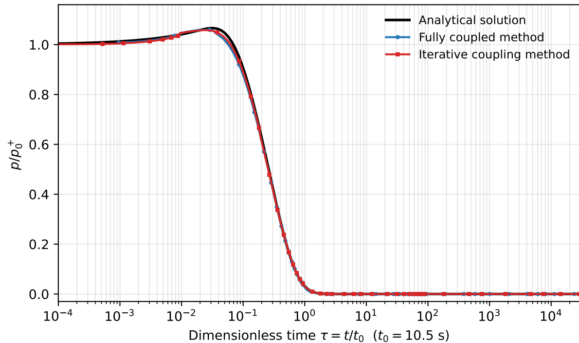
Fracture-continuum pressure
