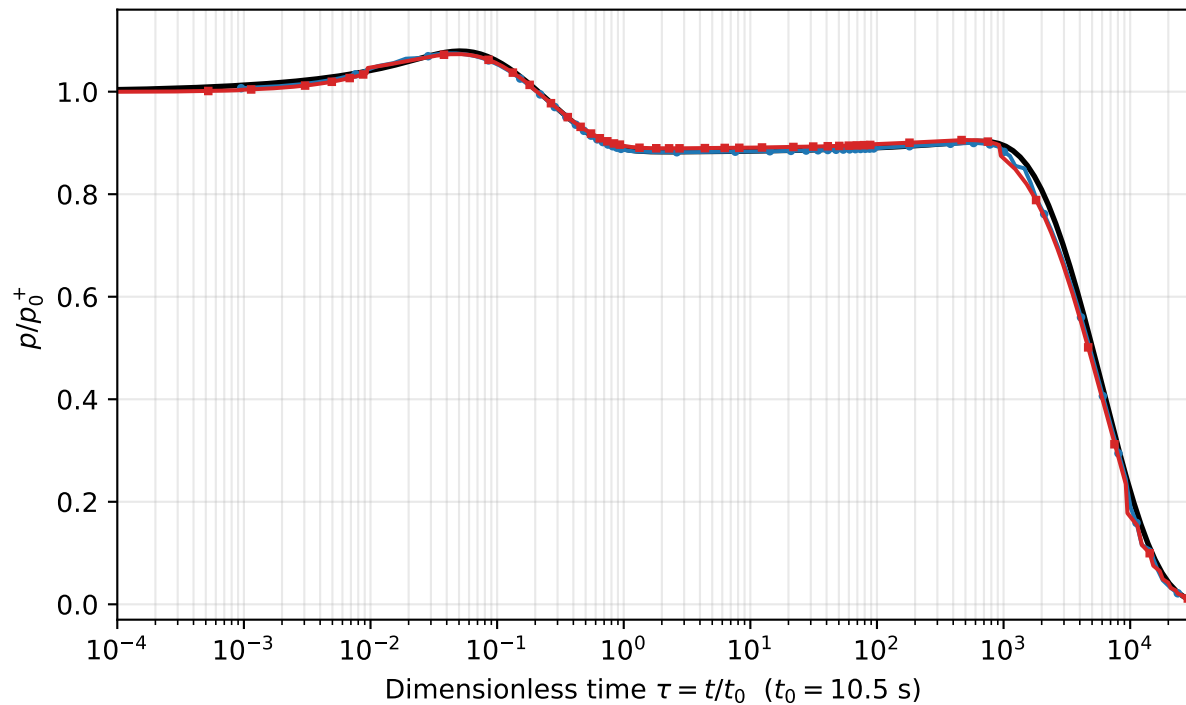
Matrix-continuum pressure
