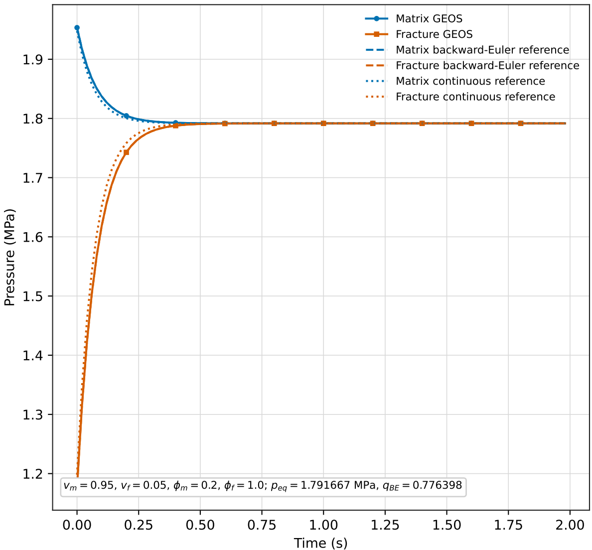
A0 unequal-volume pressure exchange
