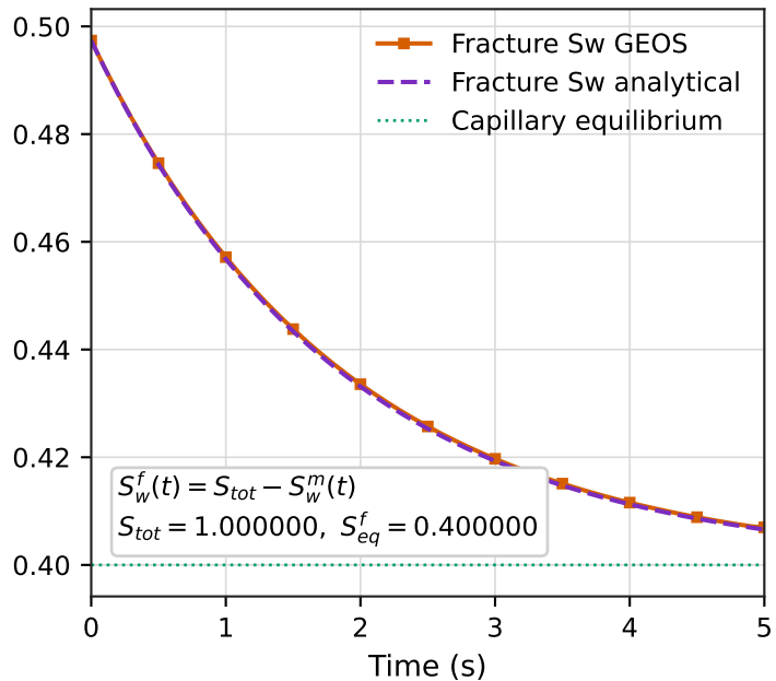
Fracture water saturation
