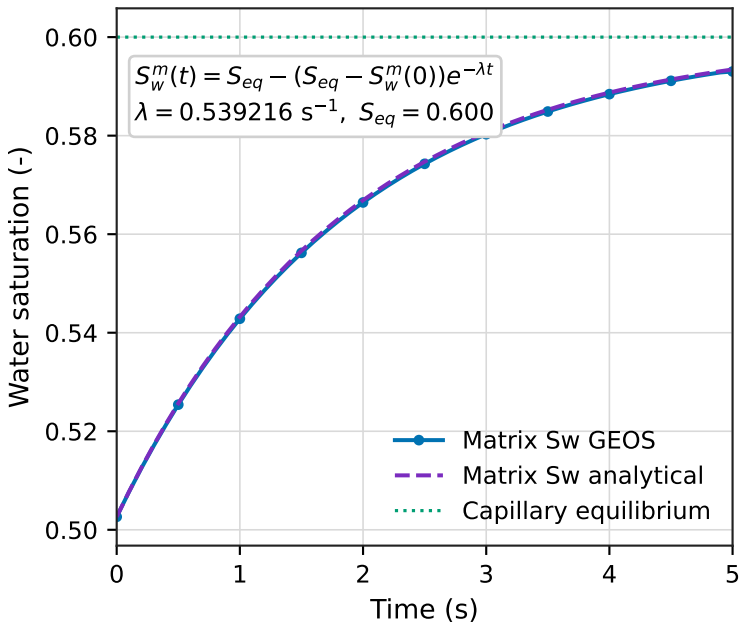
Matrix water saturation
