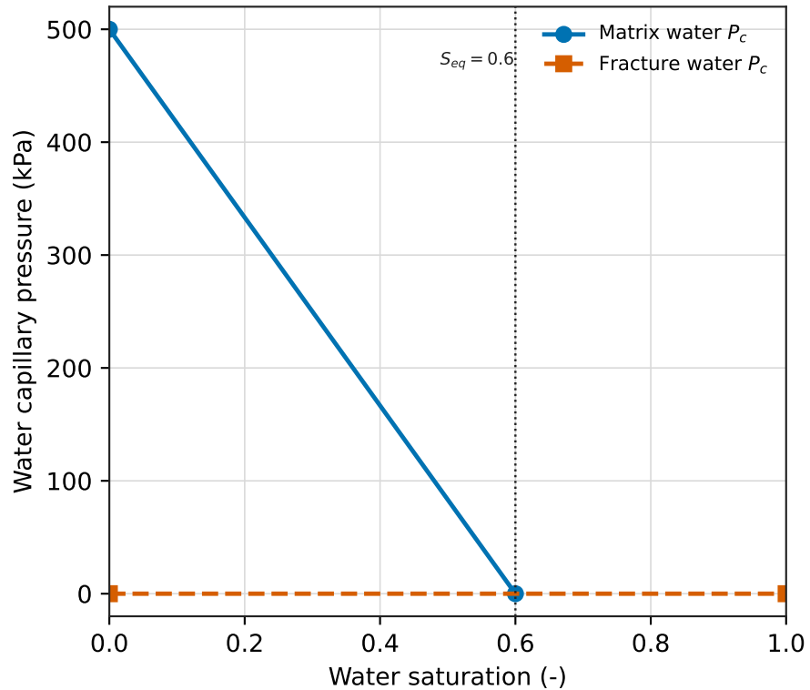
Capillary pressure
