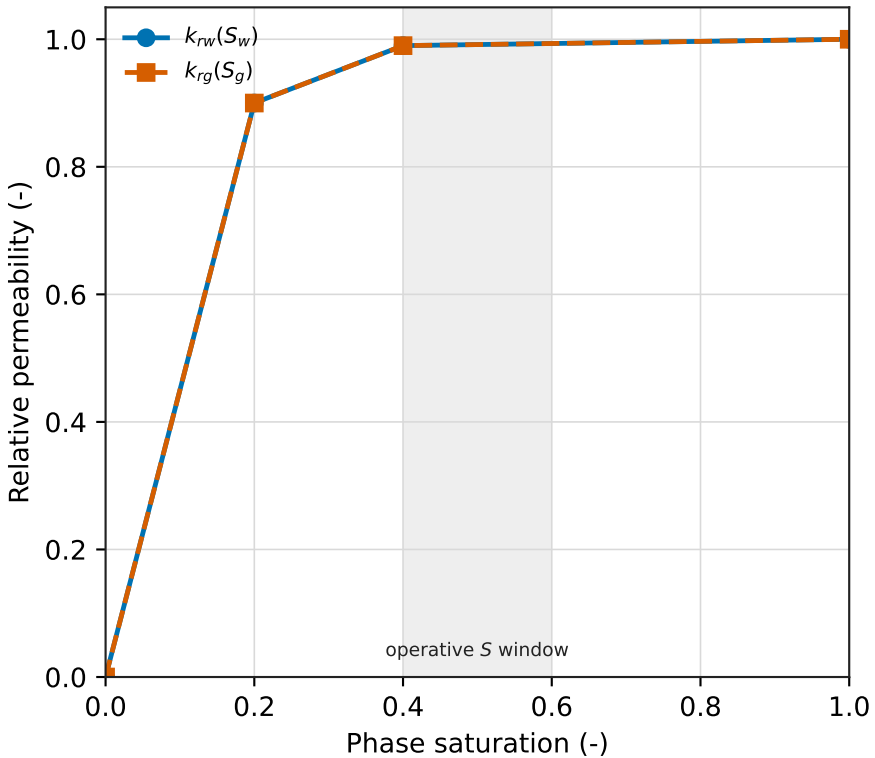
Relative permeability
