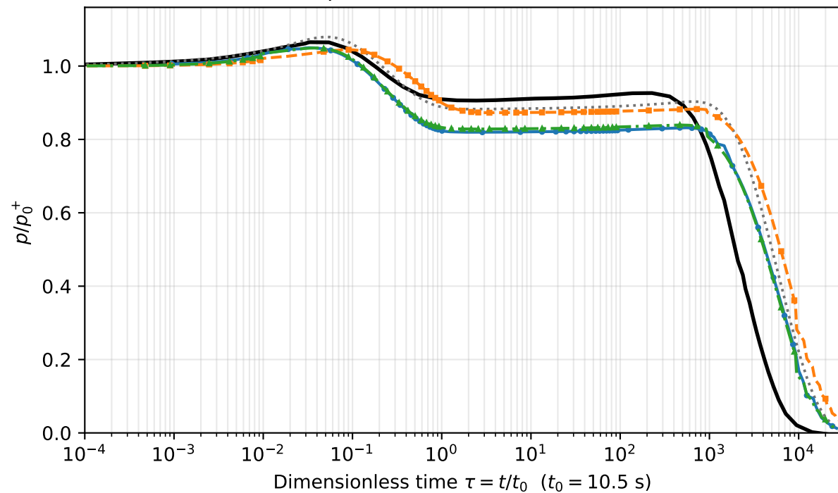
Matrix pressure at center/no-flow axis
