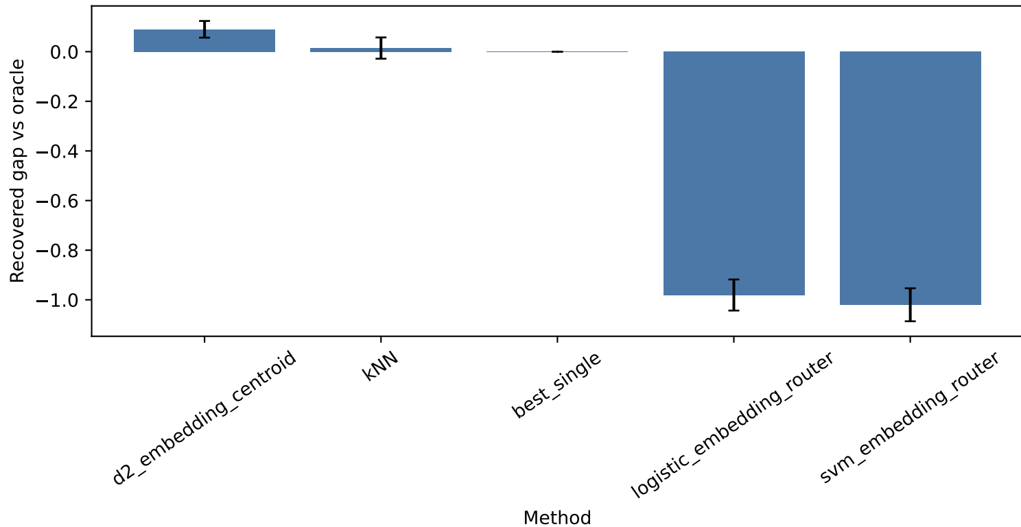
Seed Stability
