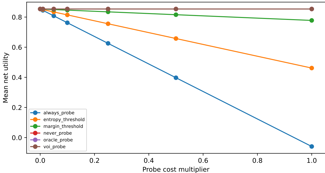
ProbeRoute++ Probe-Cost Sensitivity
