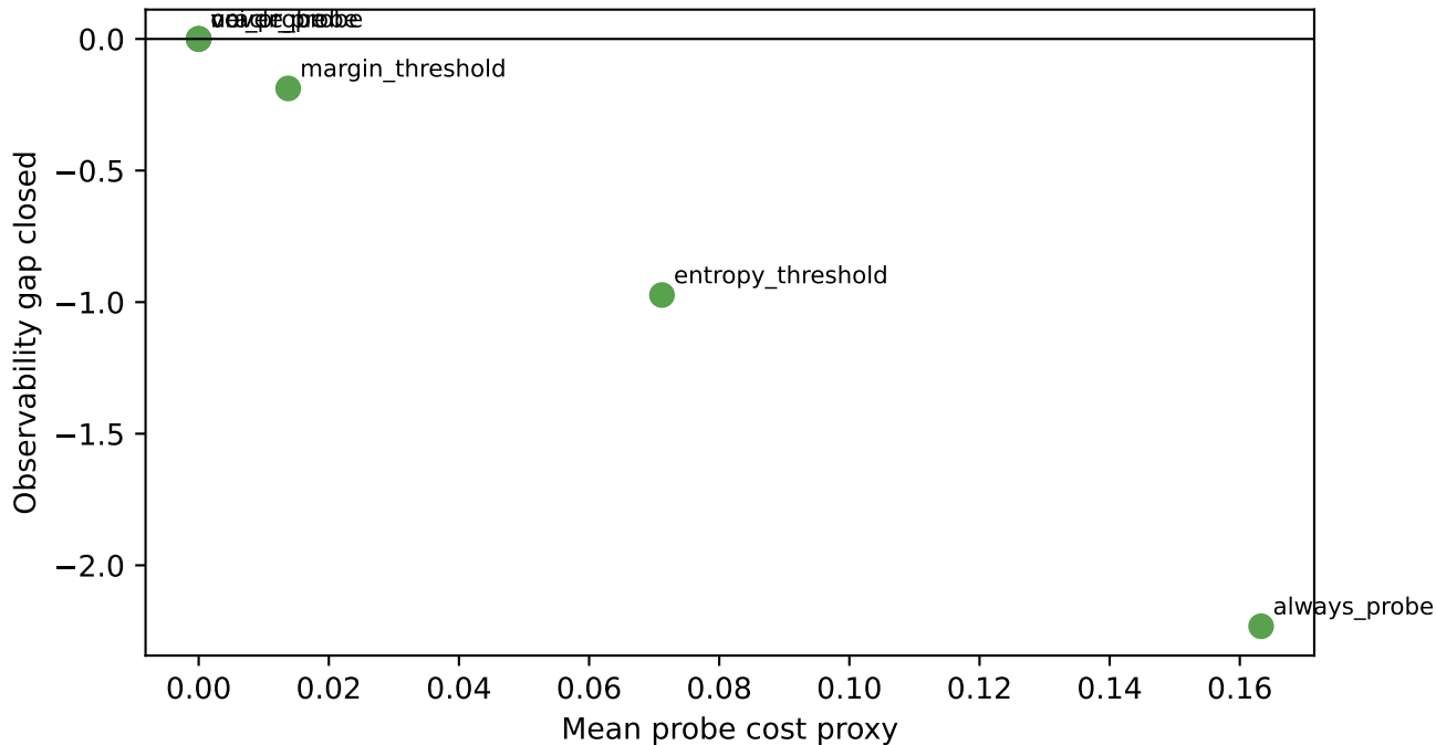
ProbeRoute++ Gap Closed vs Probe Cost
