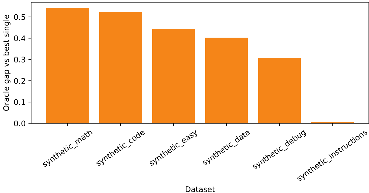
Synthetic Oracle Gap by Dataset
