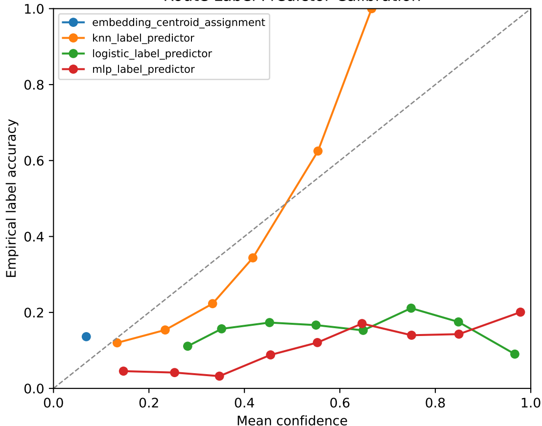
Route Label Predictor Calibration
