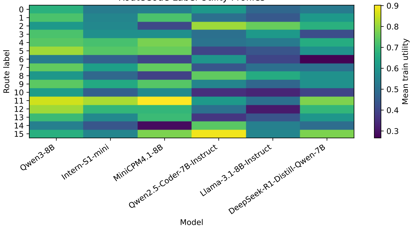
RouteCode Label Utility Profiles
