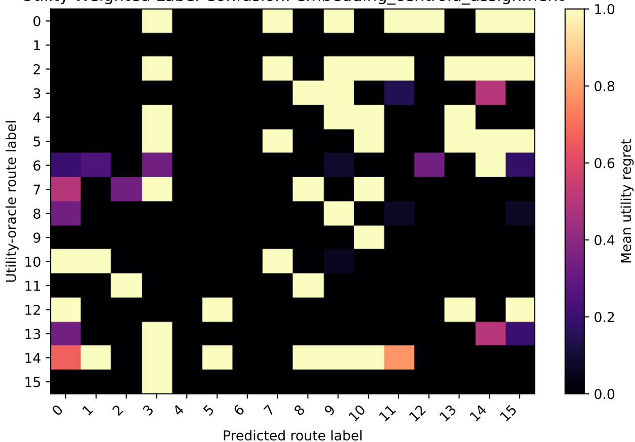
Utility-Weighted Label Confusion: embedding_centroid_assignment
