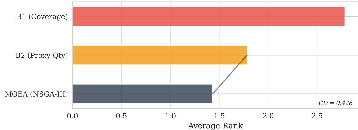
Critical Difference Diagram (Nemenyi post-hoc)
