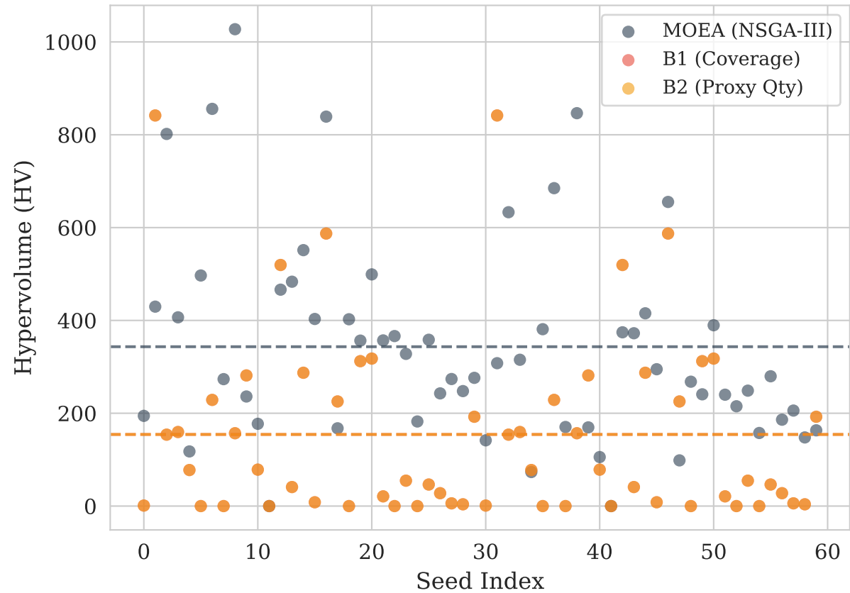
Per-Seed HV — Group S1
