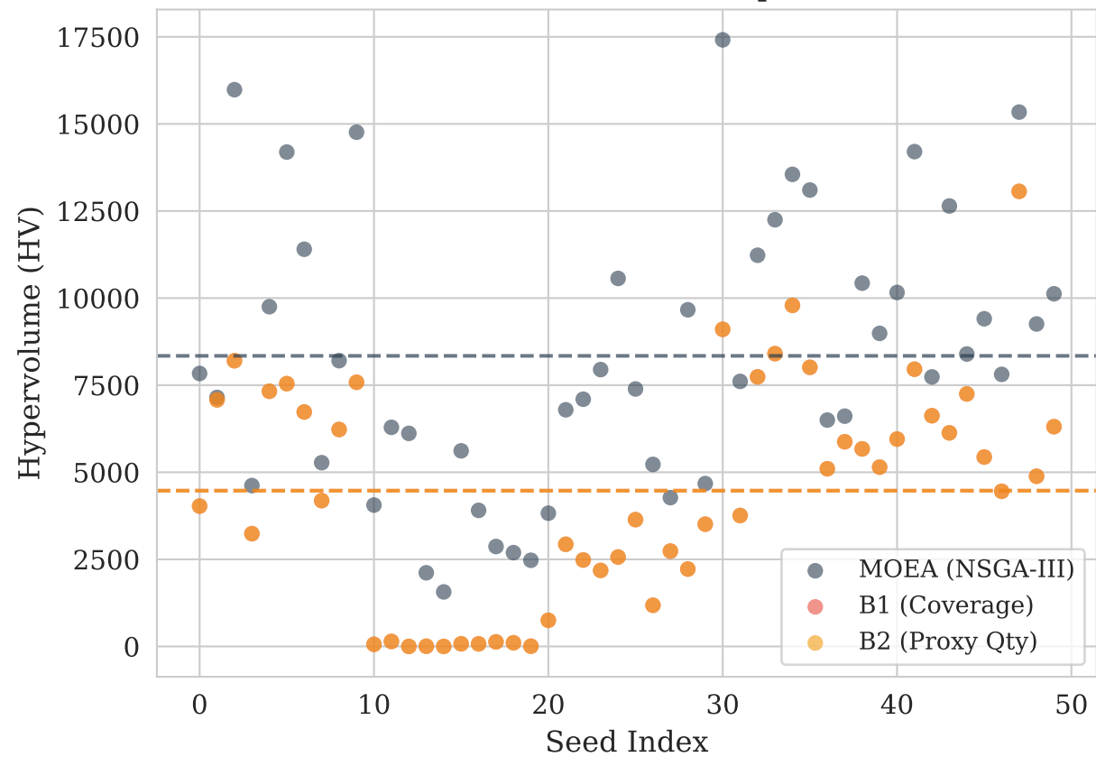
Per-Seed HV — Group S4
