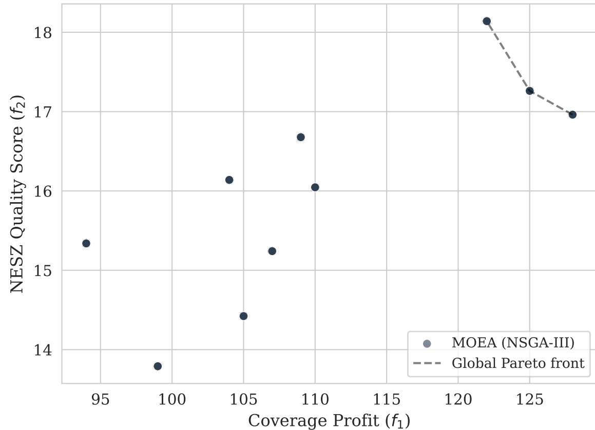
Pareto Front Comparison — Group S5
