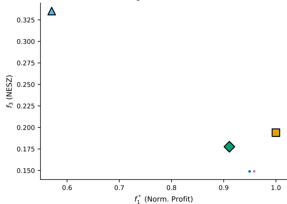
(b) f_1^* - f_3 , S4 ( N = 500 )
