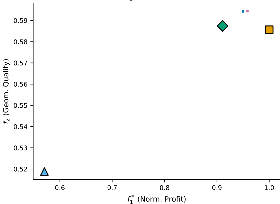
(a) f_1^* - f_2 , S4 ( N = 500 )
