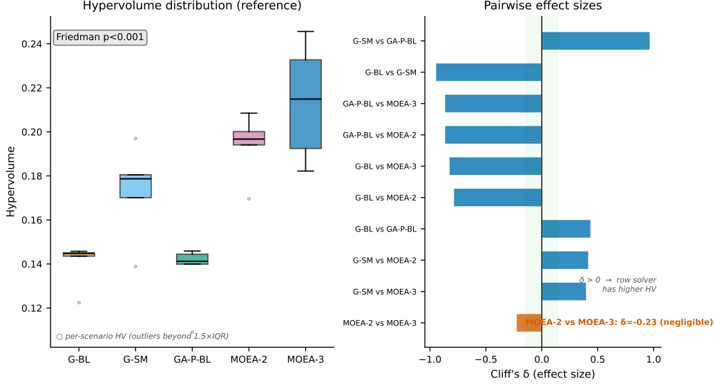
Figure 4: Statistical validation: (left) hypervolume distribution; (right) pairwise Cliff's \delta effect sizes
