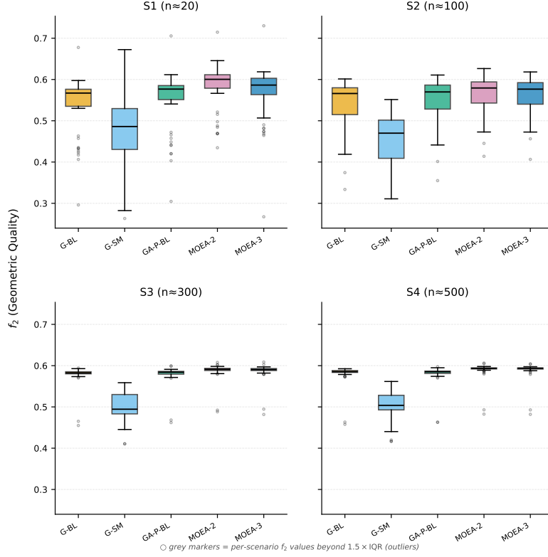
Figure 2: Geometric quality ( f_2 ) by scenario group and solver
