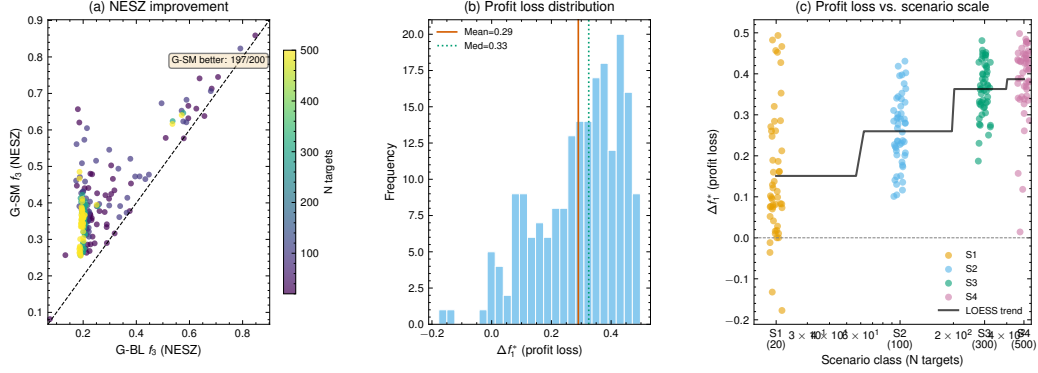
Figure 3: Effect of squint-aware scheduling: (a) f_3 scatter; (b) \Delta f_1^* histogram; (c) \Delta f_1^* vs. N with LOESS trend
