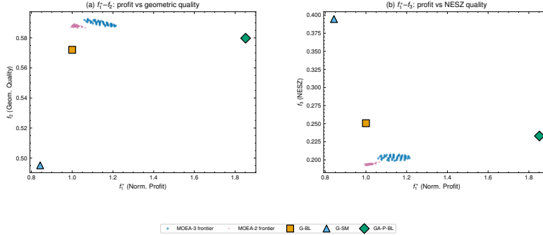
Figure 1: Pareto front on a representative S4 scenario ( N = 500 ): MOEA-3 frontier (solid, dark) with MOEA-2 overlay (light) and baseline solver markers. Panel (a): f_1^* - f_2 ; Panel (b): f_1^* - f_3 .
