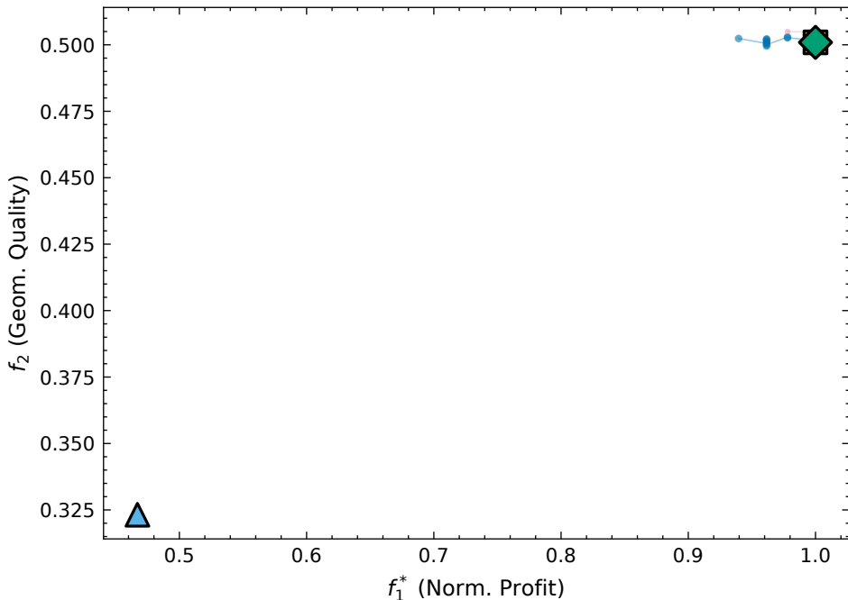
(a) f_1^* - f_2 : profit vs geometric quality
