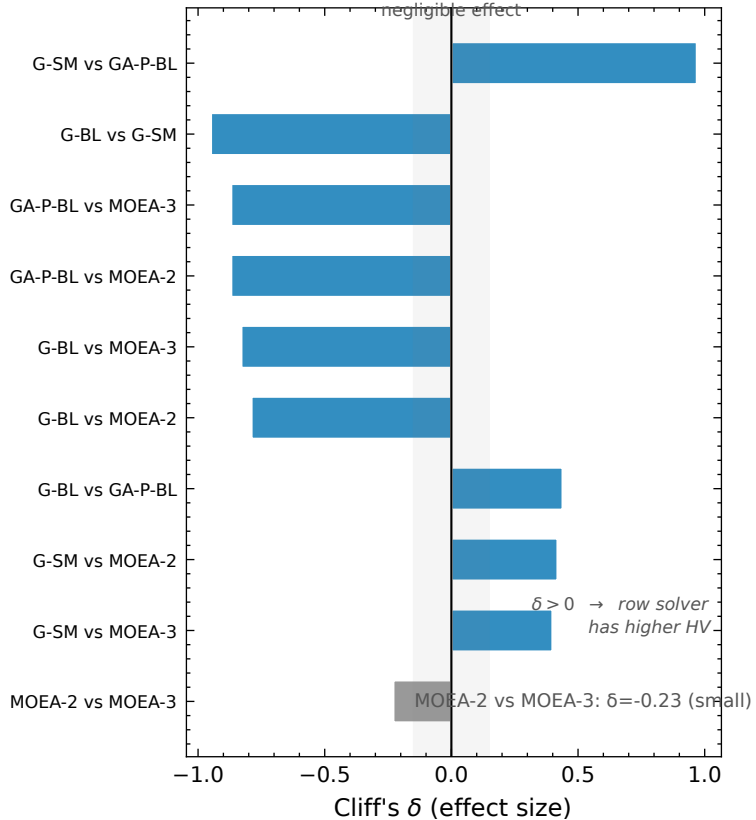
Pairwise effect sizes
