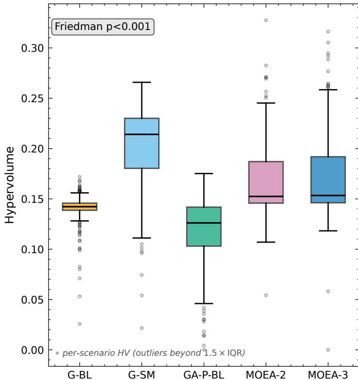
Hypervolume distribution (reference)
