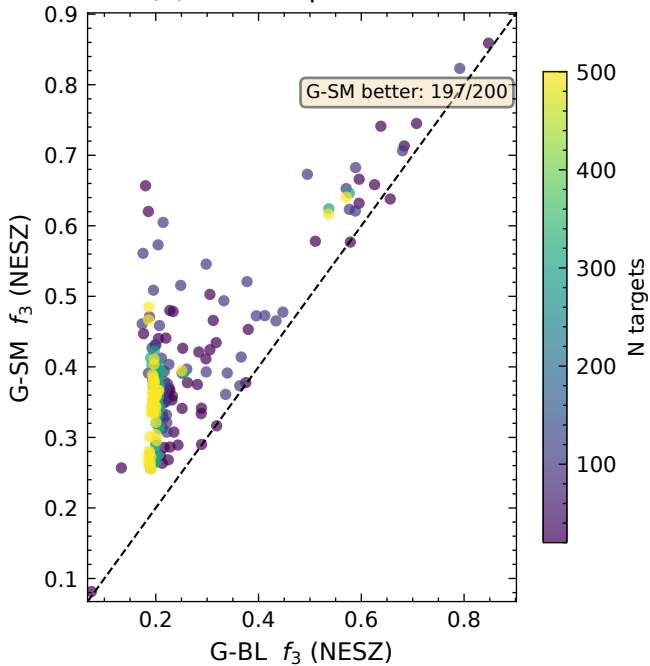
(a) NESZ improvement
