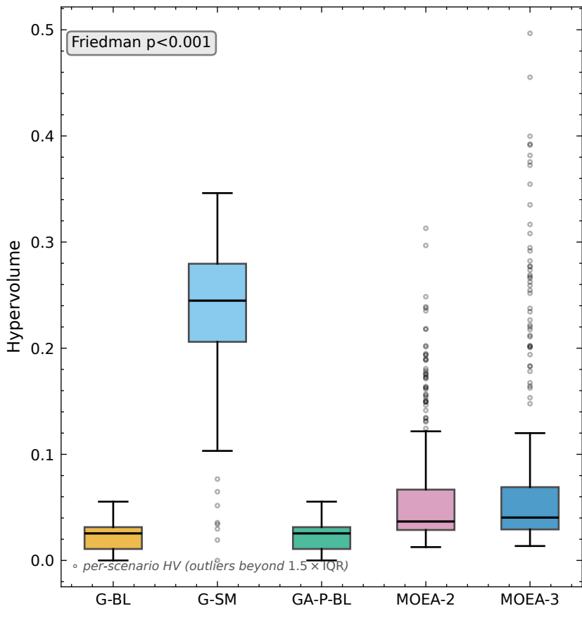
Hypervolume distribution (reference)
