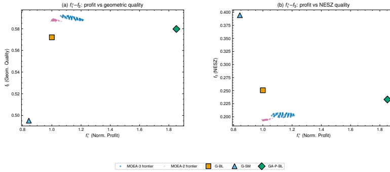
Figure 1: Pareto front on a representative S4 scenario ( N = 500 ): MOEA-3 frontier (solid, dark) with MOEA-2 overlay (light) and baseline solver markers. Panel (a): f_1^*-f_2 ; Panel (b): f_1^*-f_3 .
