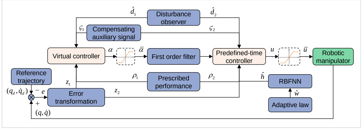
图 1 The structure of the proposed controller
