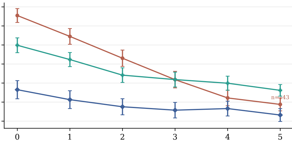
Reproduction 2 (OpenWebText training)
