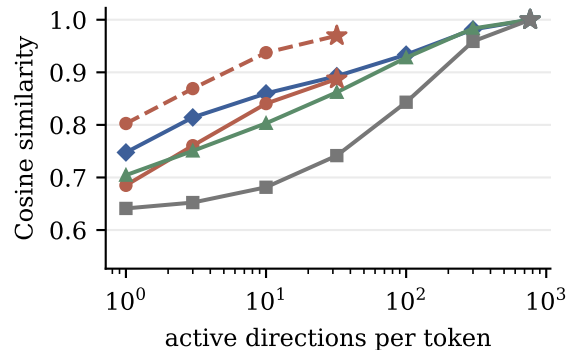
GPT-2 Small
