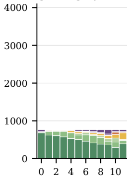
GPT-2 small
