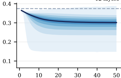
GPT-2 Small
