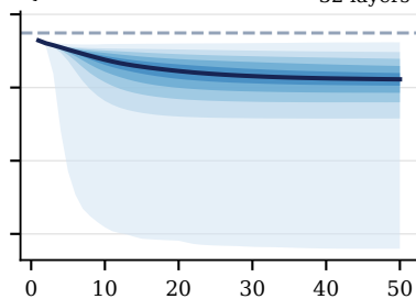
Qwen 3.5 9B
