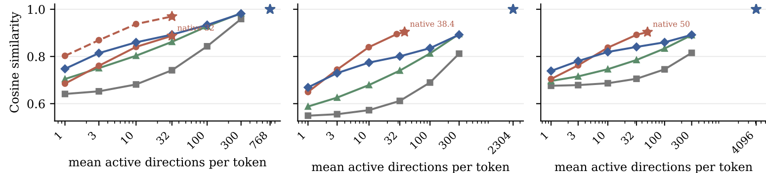
GPT-2 Small
