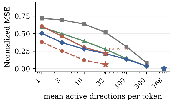
GPT-2 Small
