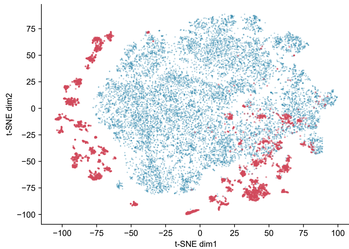
ESM2 650M
