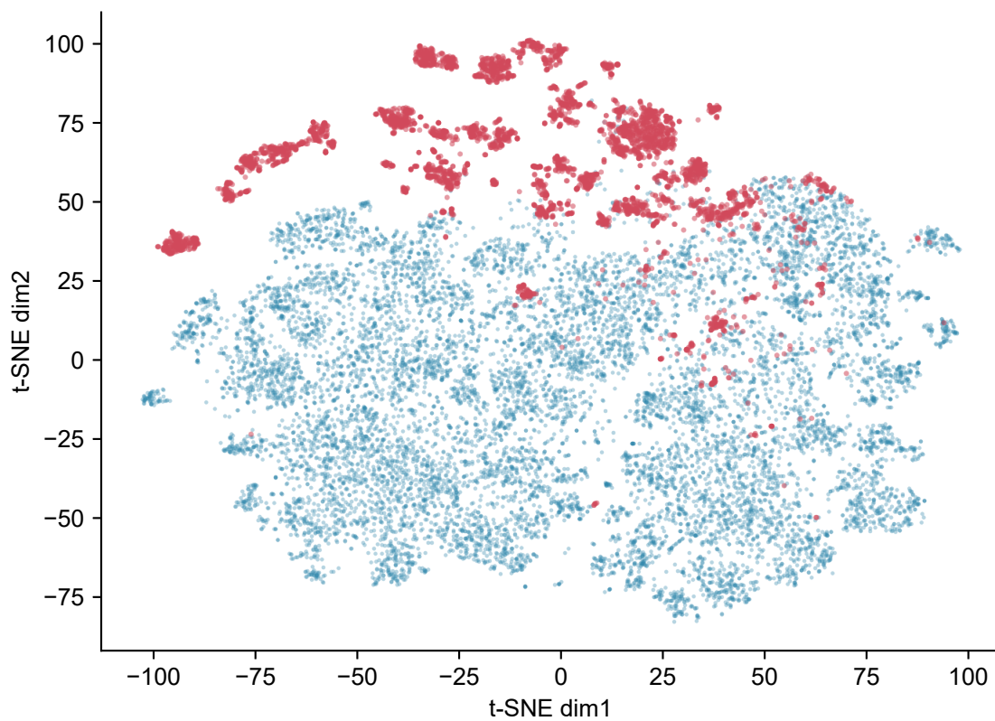
ESM2 650M
