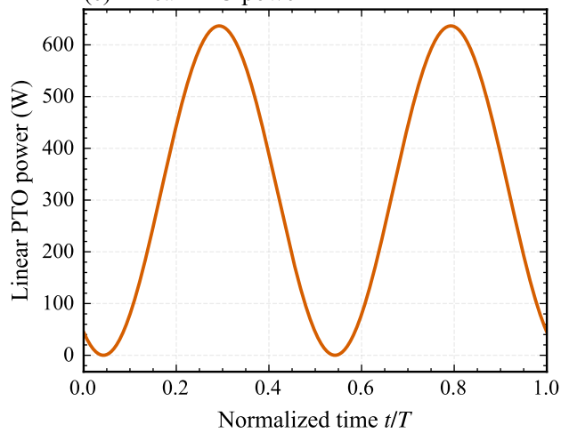
(c) Linear PTO power
