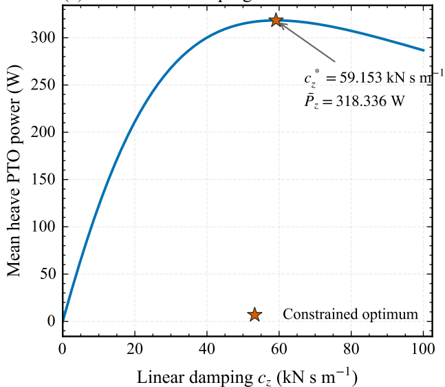
(a) Linear PTO damping
