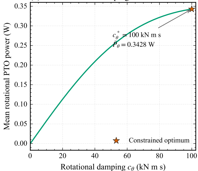
(b) Rotational PTO damping
