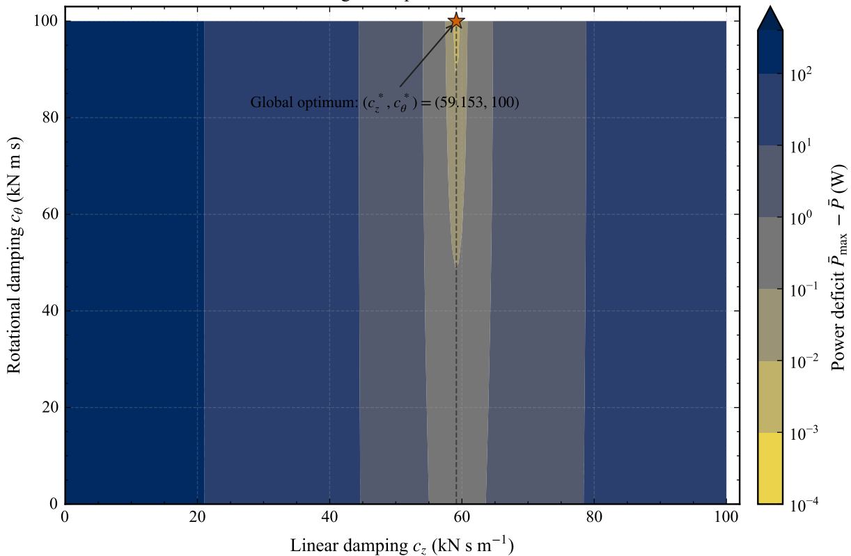
Power deficit from the constrained global optimum
