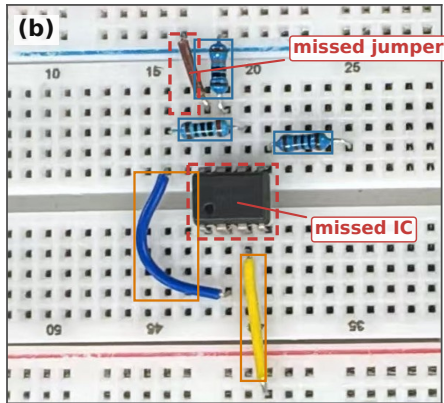
180° rotation IC and one jumper missed
