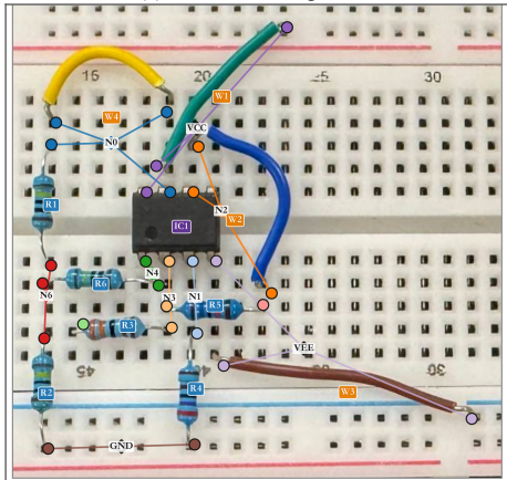
(a) hole-level assignment
