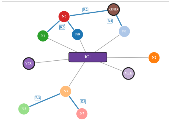
(b) component-net graph
