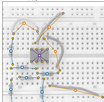
(c) pin-level structure
