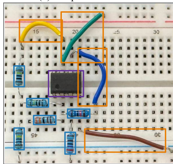
(b) component instances
