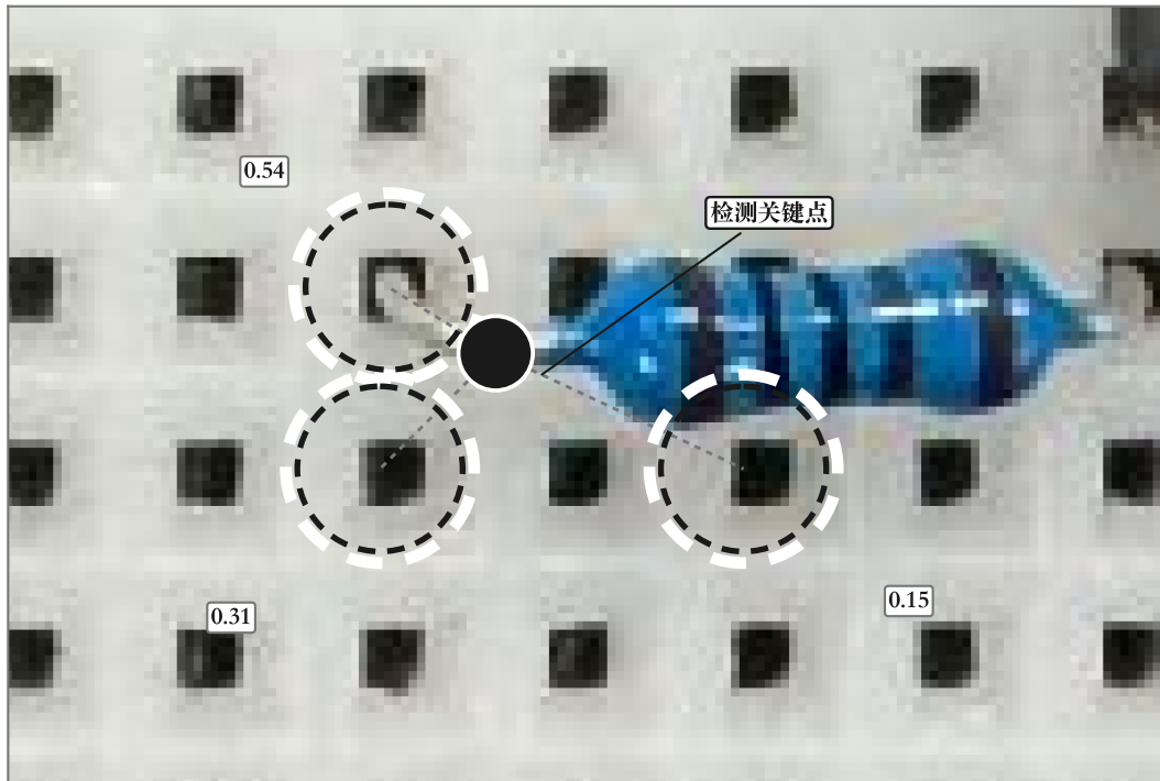
(a) 低置信引脚：候选孔位待确认
