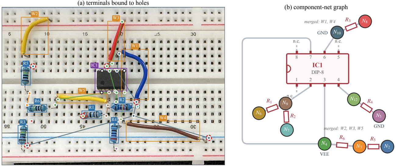
Fig. 5. Topology readout on a second board, produced by one run of the full pipeline. (a) Every detected terminal is bound to a hole and colored by the net it joins; thin links connect the terminals of one net, and dashed red rings mark the six terminals the mapper itself flagged as ambiguous. (b) The resulting component-net graph, drawn from the exported netlist with the same net colors: nets are nodes, a two-terminal component is an edge between the two nets it joins, and the DIP-8 package keeps a node of its own with numbered pins because it spans more than two nets. Twelve components and 30 terminals resolve into ten nets; the five jumper wires contribute no edges but merge strips, and the nets they created are tagged with the wires responsible. Pins 1, 5 and 8 of the package reach single-terminal nodes and are reported as unconnected.
