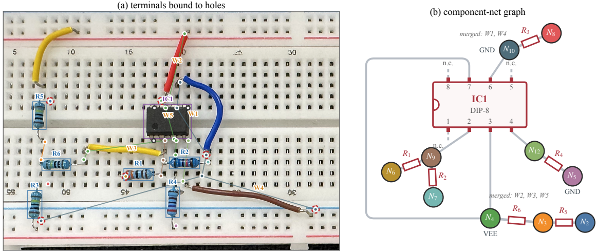
Fig. 4. Topology readout on a second board. (a) Terminals are bound to holes and colored by electrical net; dashed rings denote ambiguous assignments. (b) The exported component-net graph uses the same colors, providing a direct visual correspondence between image evidence and symbolic structure.
