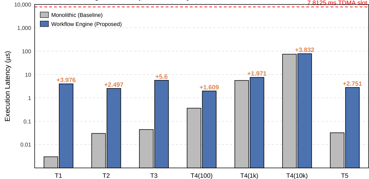
Figure 3. Comparative Analysis of Execution Overhead
