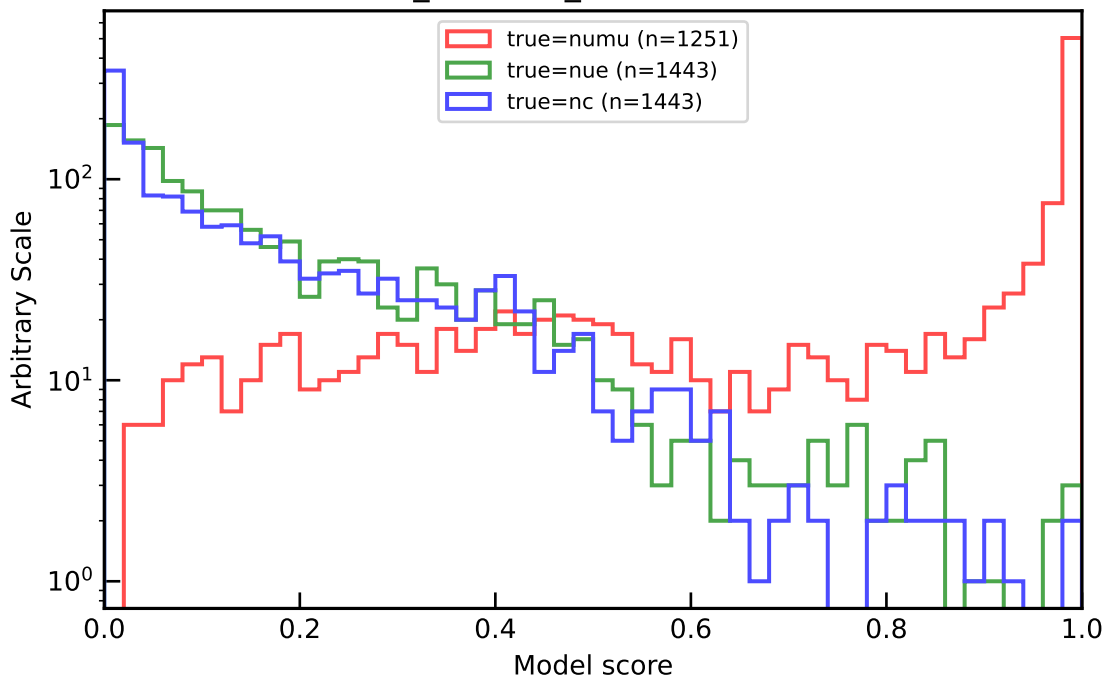
fea6+wfs_wav: mu_like score distribution
