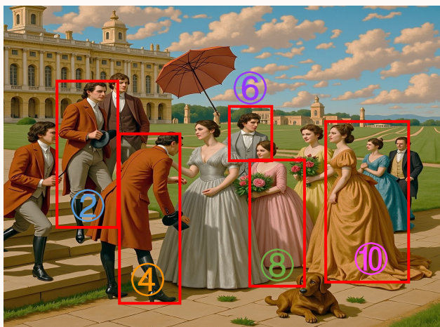
FLUX ControlNet
