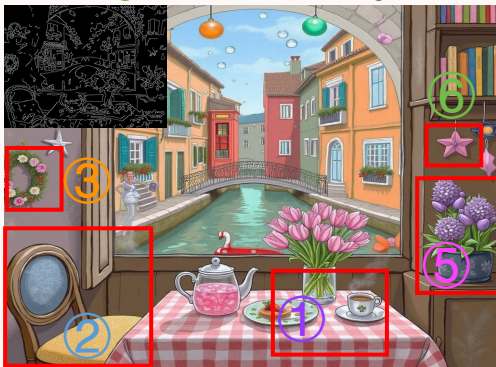
FLUX ControlNet
