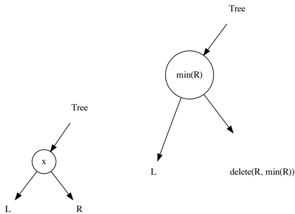
(a) Before delete x .
