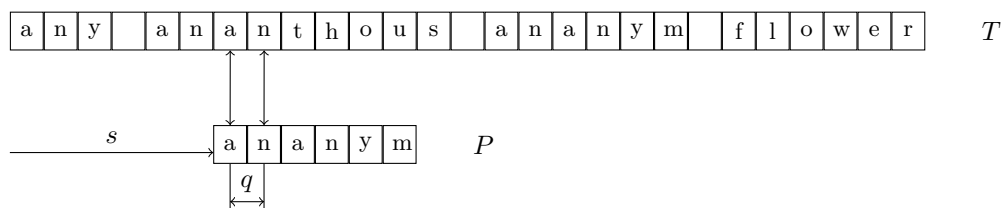
(b) Move s = 4 + 2 = 6 .
