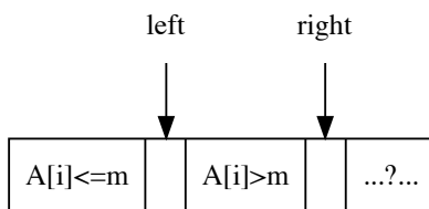
Figure 1: All A[i] \leq m where 0 \leq i < left ; while A[i] > m where left \leq i < right . The rest elements are yet to be scanned.
