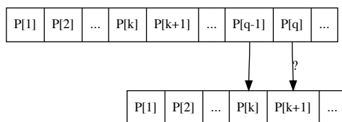
Figure 14.14: P_k is suffix of P_{q-1} , compare P[q] and P[k + 1] .
