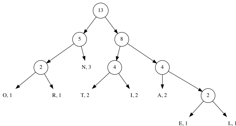
Figure 14.34: Huffman tree
