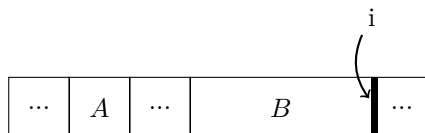
Figure 14.11: A : max sum so far; B : sum of the sub-vector ends with i .
