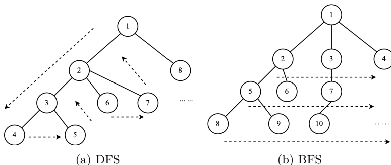
Figure 14.31: DFS and BFS.
