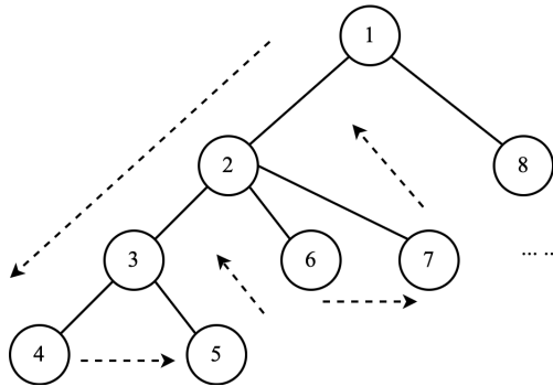
Figure 14.21: DFS search order.
