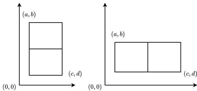
Figure 14.8: Chose the shorter center line.
