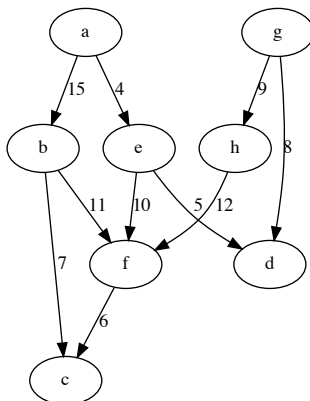
Figure 14.32: A weighted directed graph.
