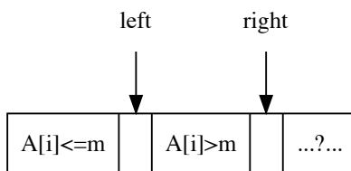
Figure 1: All A[i] \leq m where 0 \leq i < \text{left} ; while A[i] > m where \text{left} \leq i < \text{right} . The rest elements are yet to be scanned.
