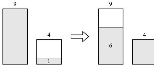
Figure 14.25: The last two steps.
