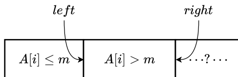
Figure 1: All A[i] \leq m where 0 \leq i < left ; while A[i] > m where left \leq i < right . The rest elements are yet to be scanned.
