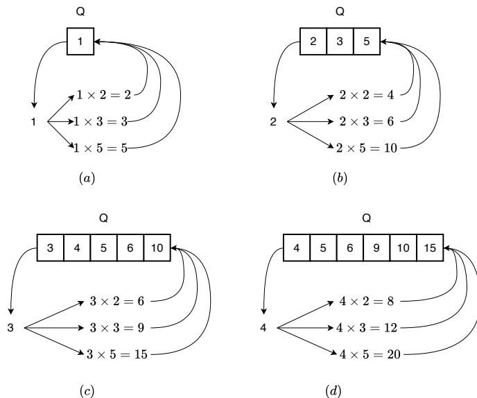
Figure 2: First 4 steps: add 1; add 2, 3, 5; add 4, 6, 10; add 9, 15, drop 6.
