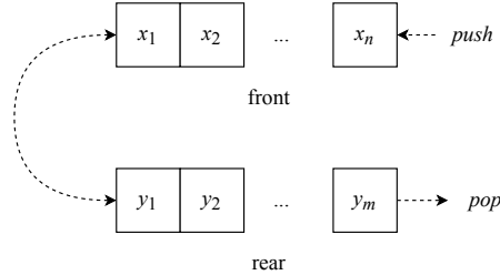
Figure 11.6: paired-array queue.
