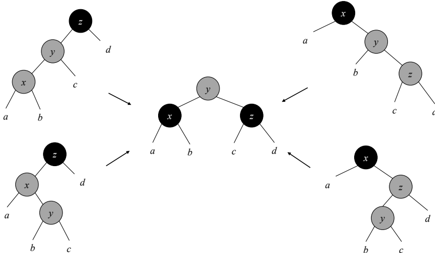
Figure 4.6: Fix 4 cases to the same structure.
