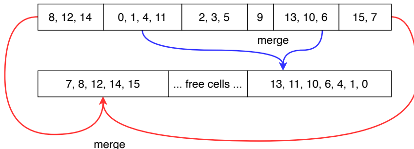
Figure 13.15: Nature merge sort
